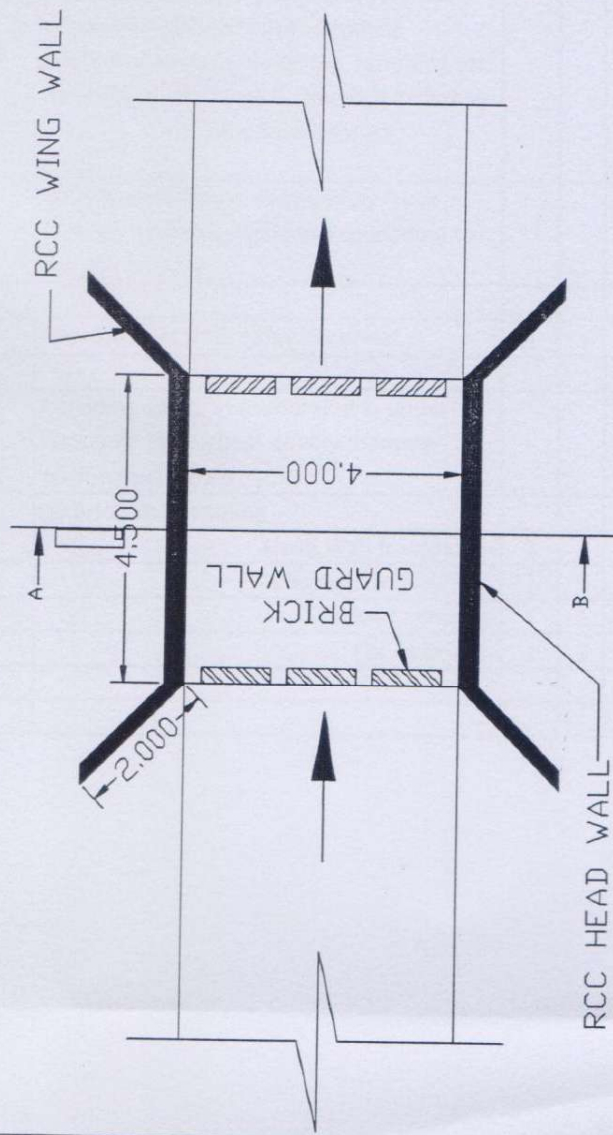
LAYOUT PLAN
