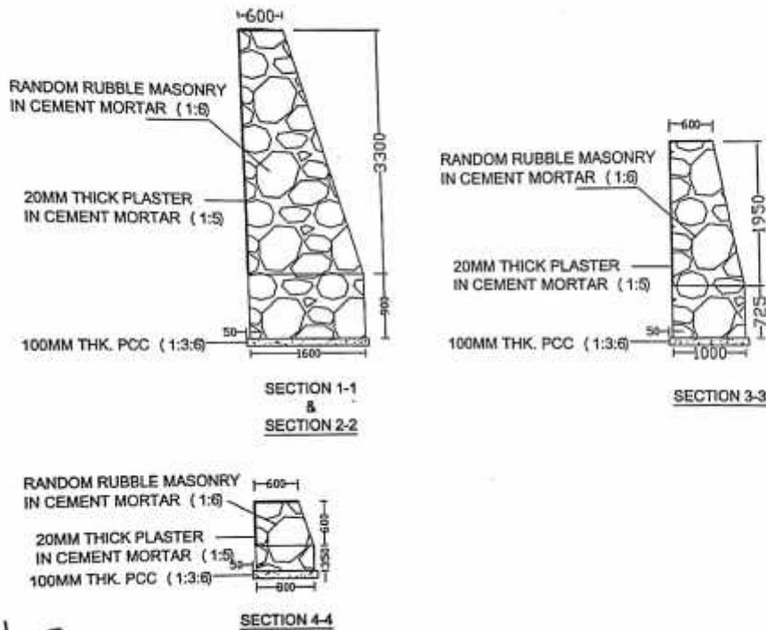
SECTION OF R.R.M WALL - XY
