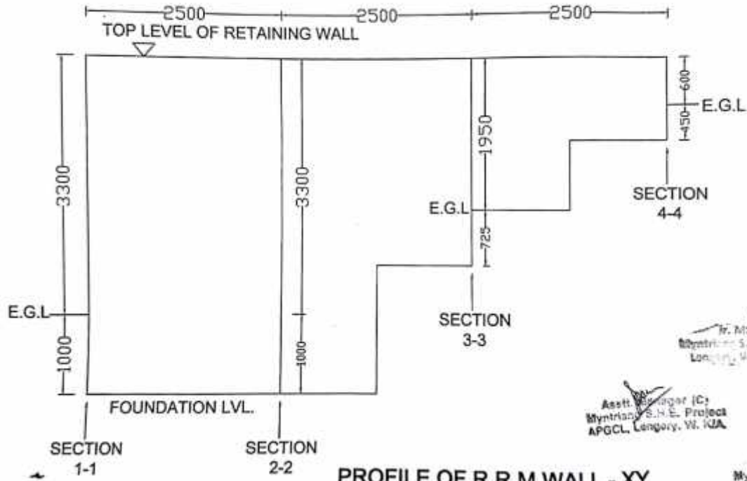
PROFILE OF R.R.M WALL - XY
