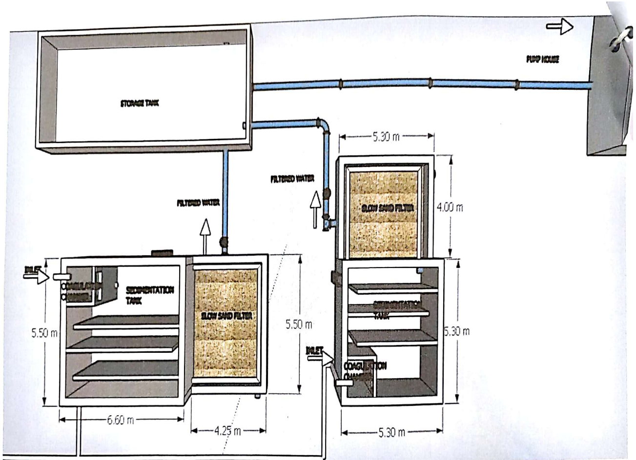
EXISTING WATER SUPPLY SYSTEM AT KLHEP,PUMP HOUSE,LENGERY COLONY.
