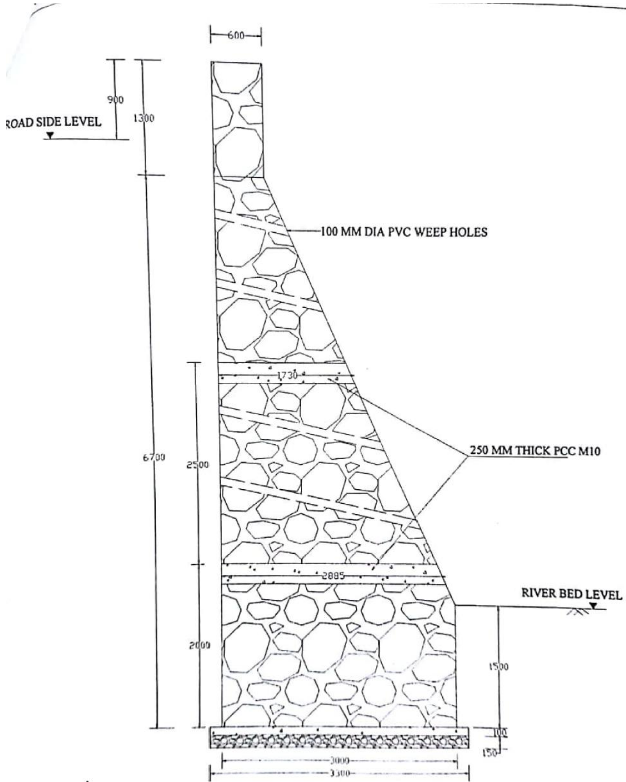
DETAILS SECTION OF LEFT BANK WING WALL
