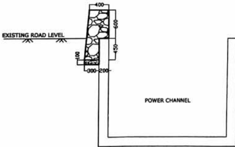
SECTION FOR CH.2050 TO 2065M
