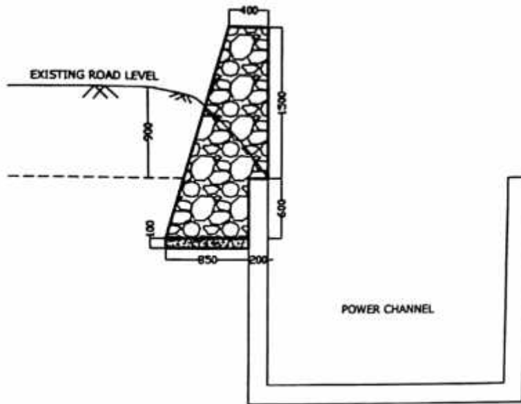
SECTION FOR CH.2917 TO 2935M
