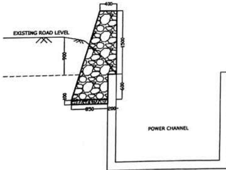
SECTION FOR CH.2130 TO 2149M
