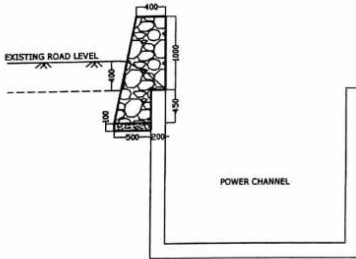
SECTION FOR CH.2910 TO 2917M
