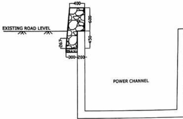
SECTION FOR CH.2900 TO 2910M
