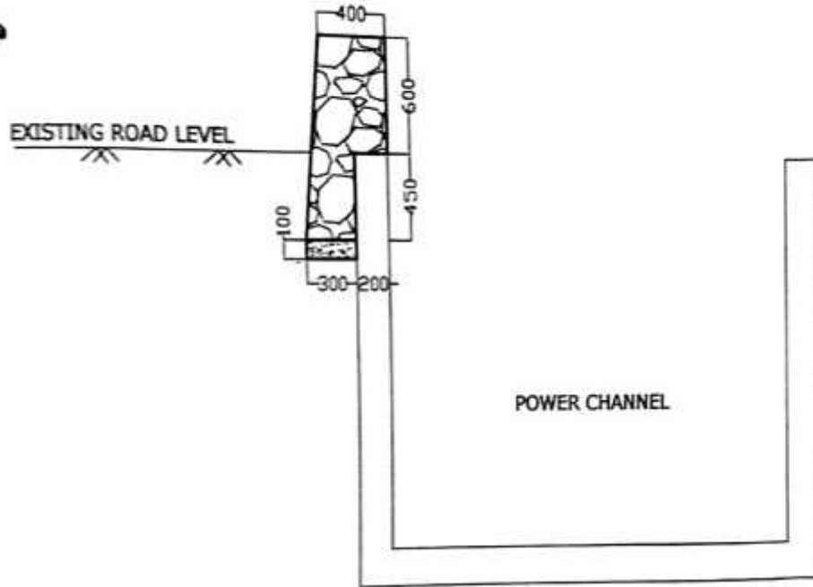
SECTION FOR CH.1747 TO 1767M
